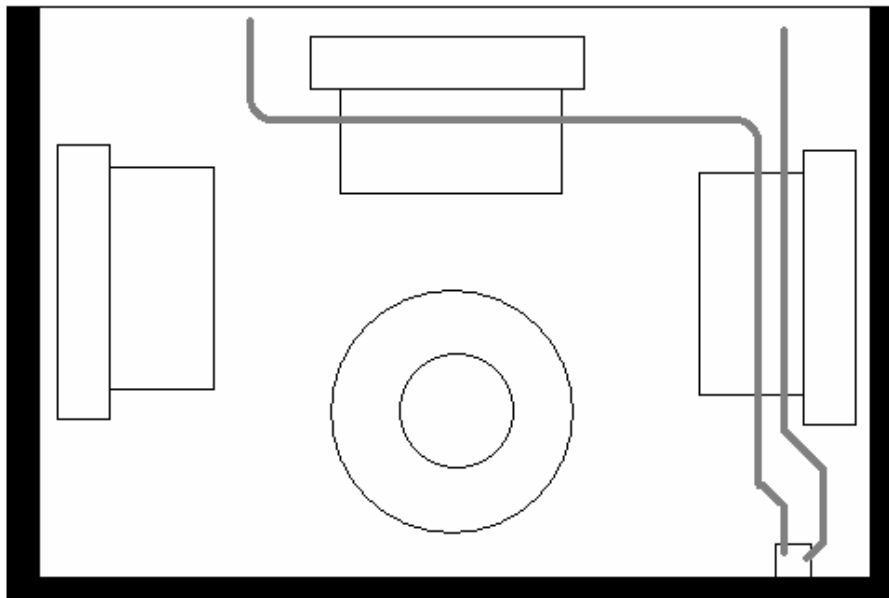
Figure 5-Shielded cable routing
