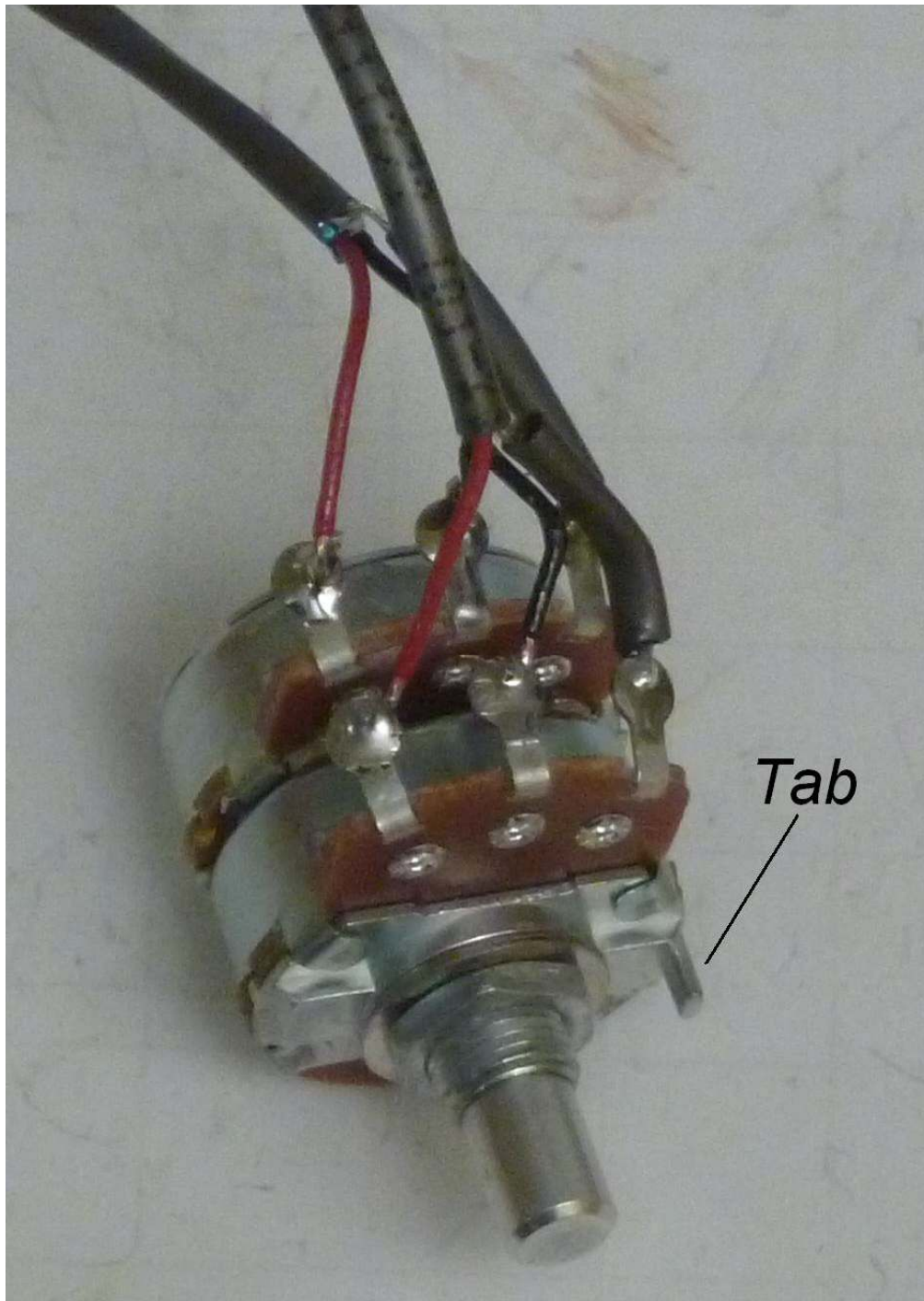
Figure 3-Connect the shielded cables to the volume control. Remember to remove the tab
