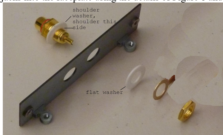
Figure 6-Hardware detail for installing the RCA Jacks and insulating washers into the faceplate Jack Installation
