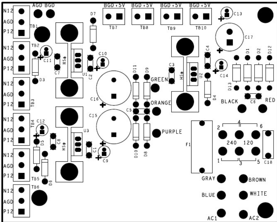
Figure 2-Component side of power supply PCB before loading
