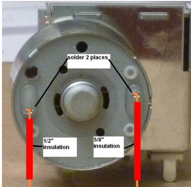
Figure 39-Motor POT wiring detail
