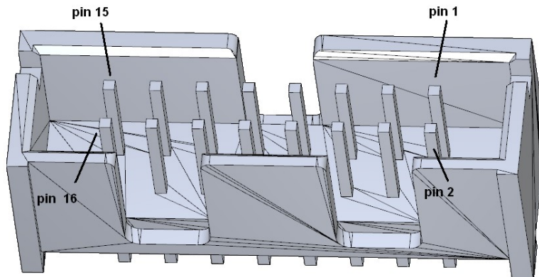
Figure 23-locating the pins on the 16 pin cable connector
