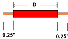
Figure 38-Motor POT wire preparation
