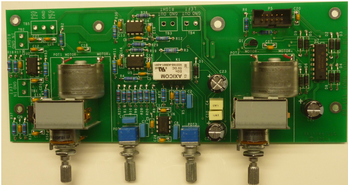
Figure 40-Completed Tone/Volume Board
