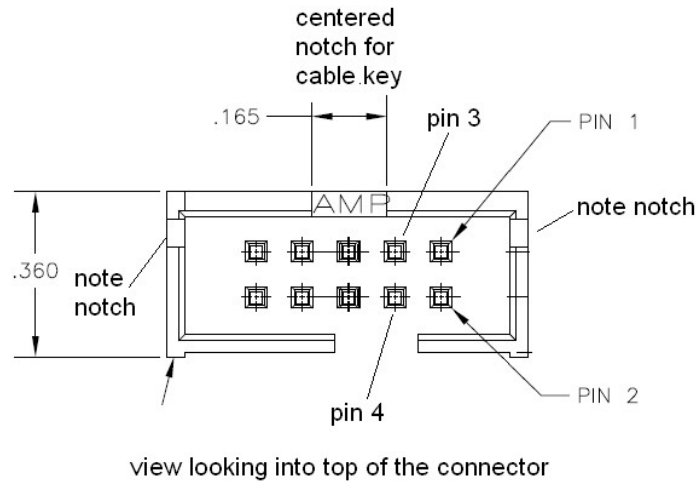
Figure 22-10 pin cable connector pinout
