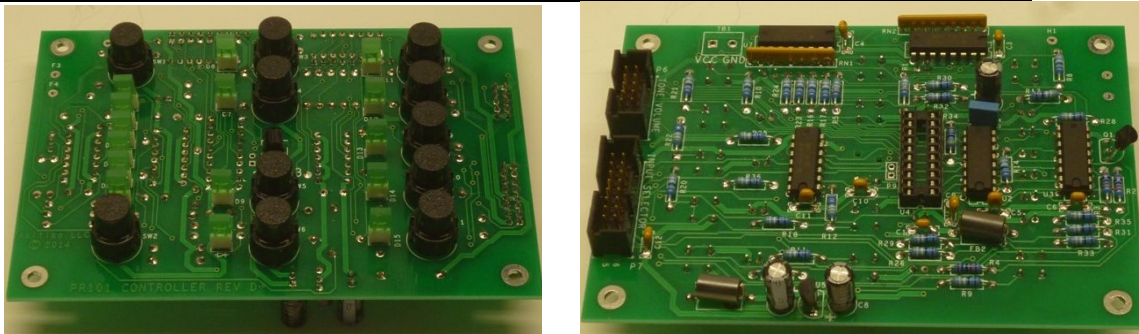
Figure 28-Completed controller, push-button and LED side and component side
