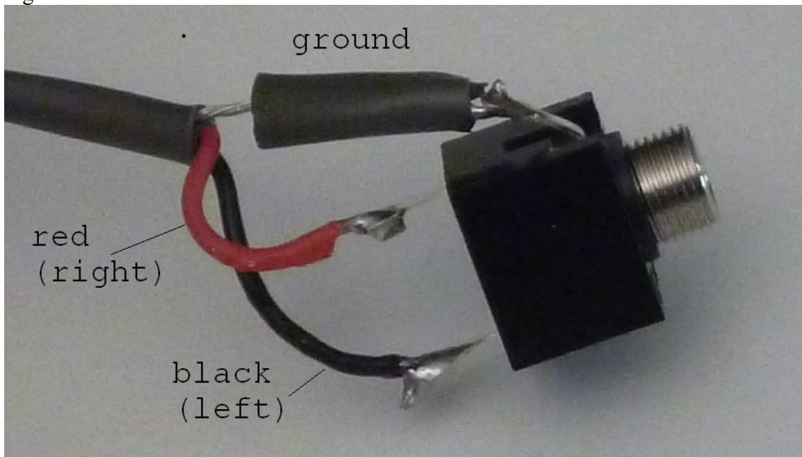
Figure 41-Connecting wires to front panel (FP) 1/8" phono jack
