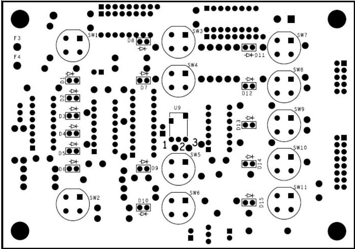
Figure 25-Switch and LED side of Controller Board
