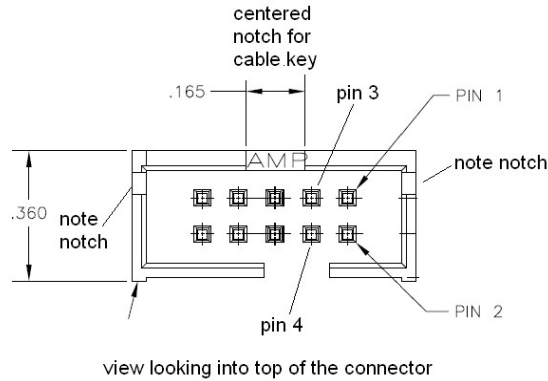
Figure 37-Identify pin 1 for proper connector installation
