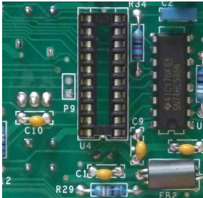
Figure 24—showing socket orientation
