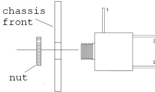
Figure 42-Inserting 1/8" jacks in the front panel
