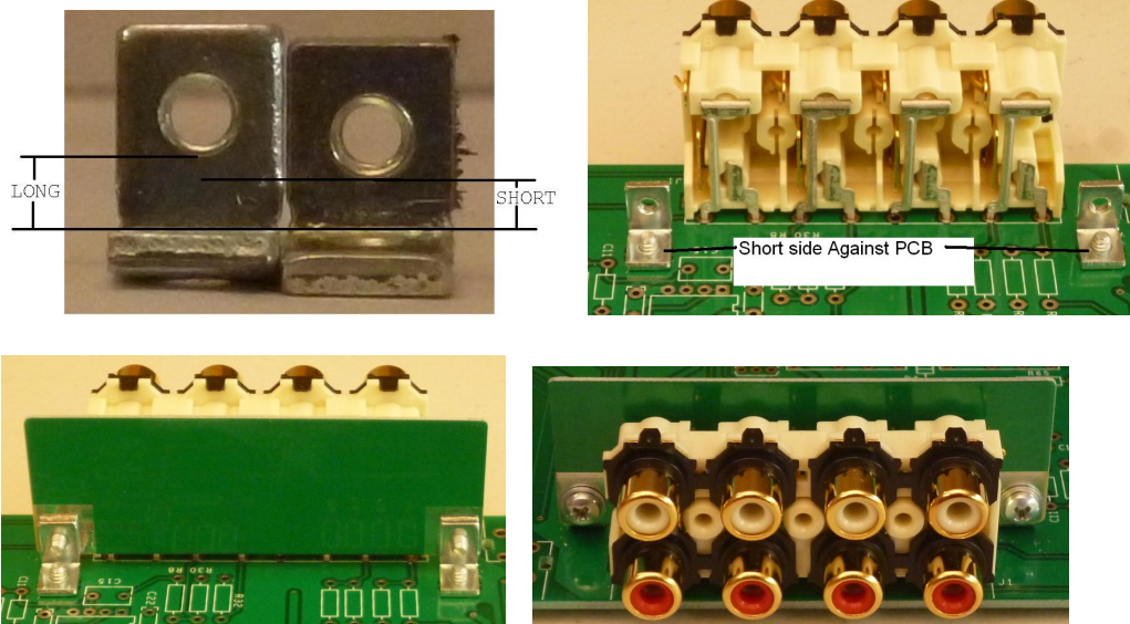
Figure 31-Mounting the input connector shield
