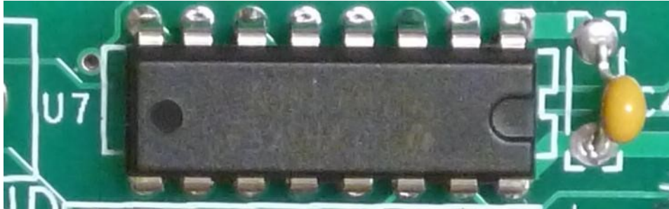
Figure 21-Insert all the IC's so that the U-shaped indent matches the silk-screen
