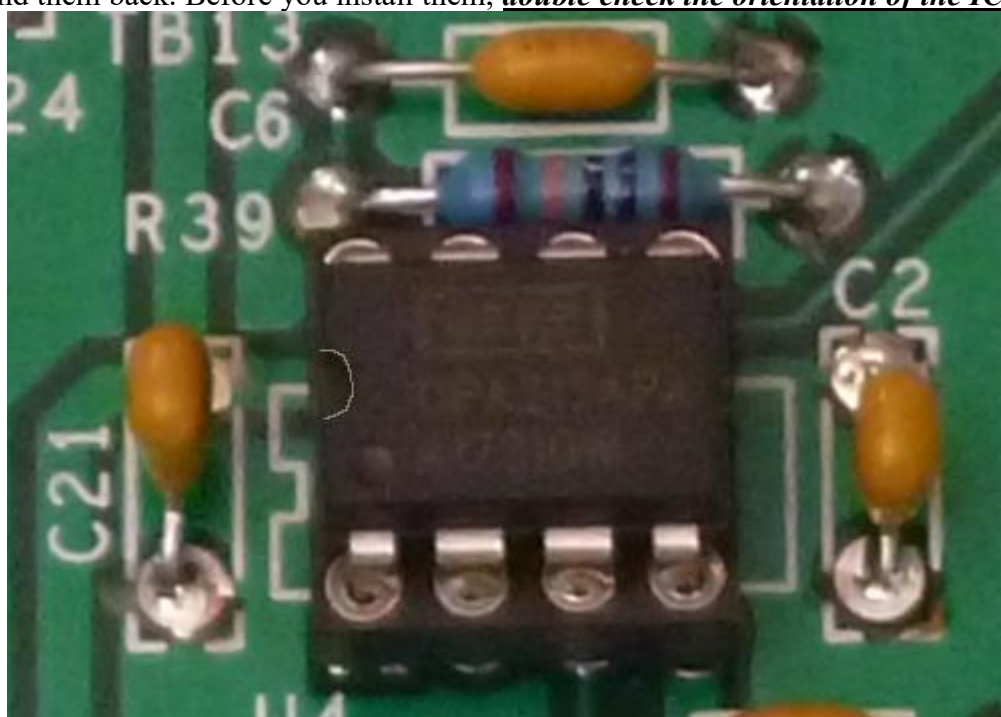
Figure 33-Insert opamp so semi-circular indentation in IC package matches silk-screen feature
