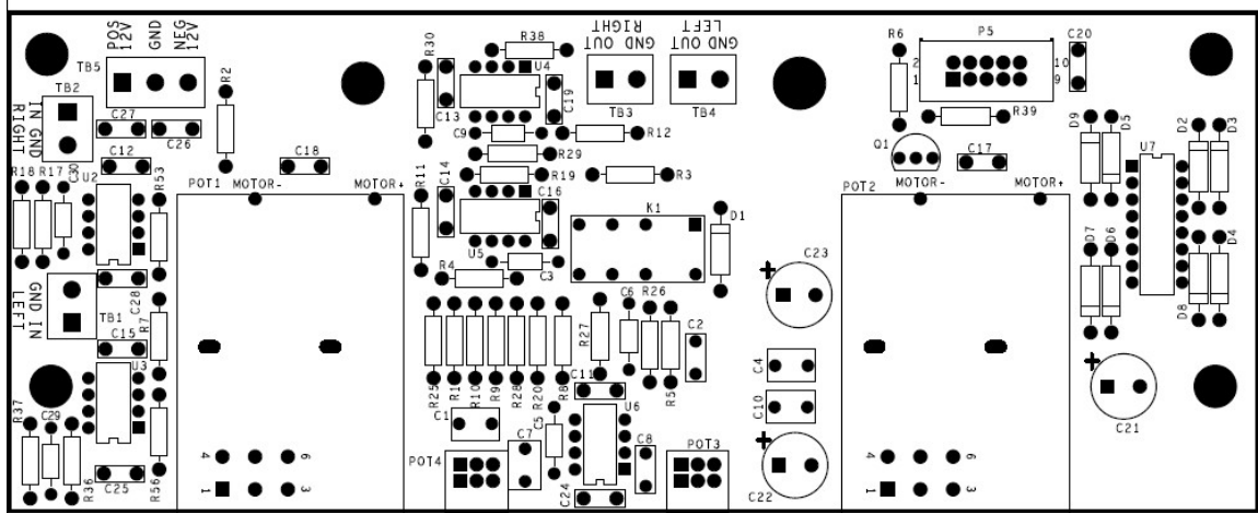
Figure 35-Silkscreen side of the Tone Volume Board shows component locations
