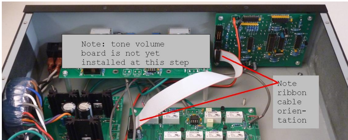
Figure 34-16 pin ribbon cable orientation and installation
