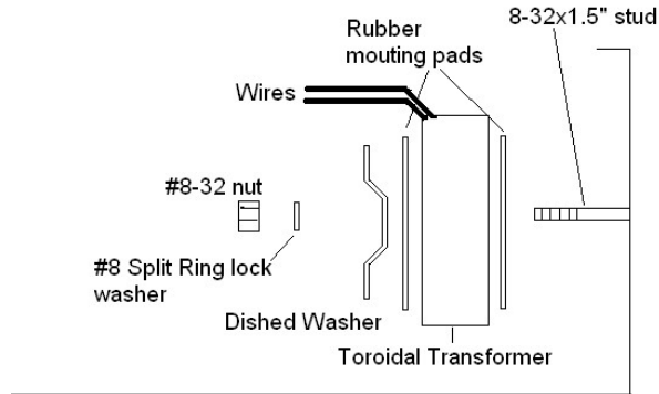
Figure 18-Fasten the transformer to the preamp right side wall
