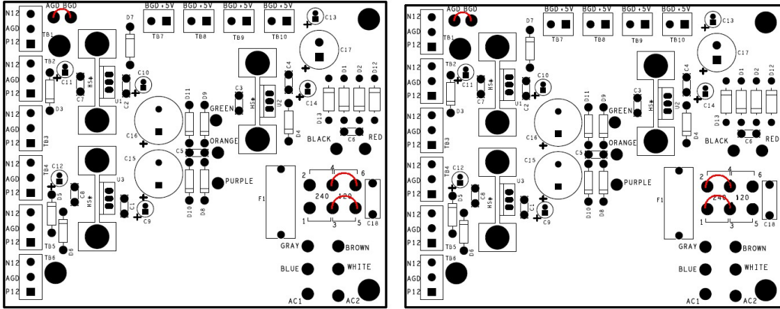
Figure 8-Jumper installation for 120 Volt Operation (left side) and 240 Volt (right side)
