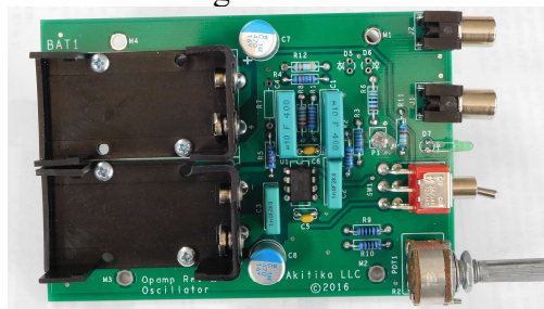
Figure 4-Battery Holder Installation
