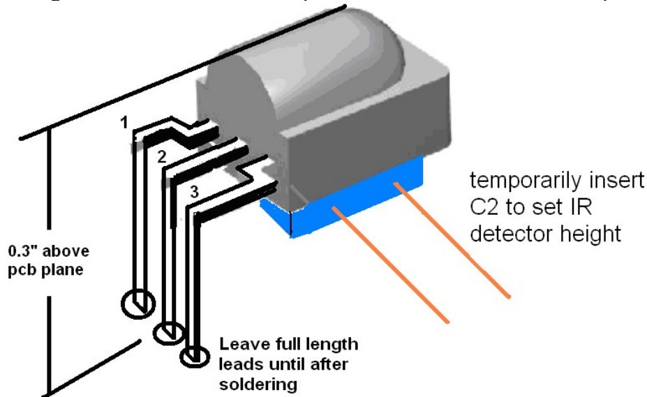
Figure 26-Infra-red detector for remote control mounts 0.3” above plane of pcb
