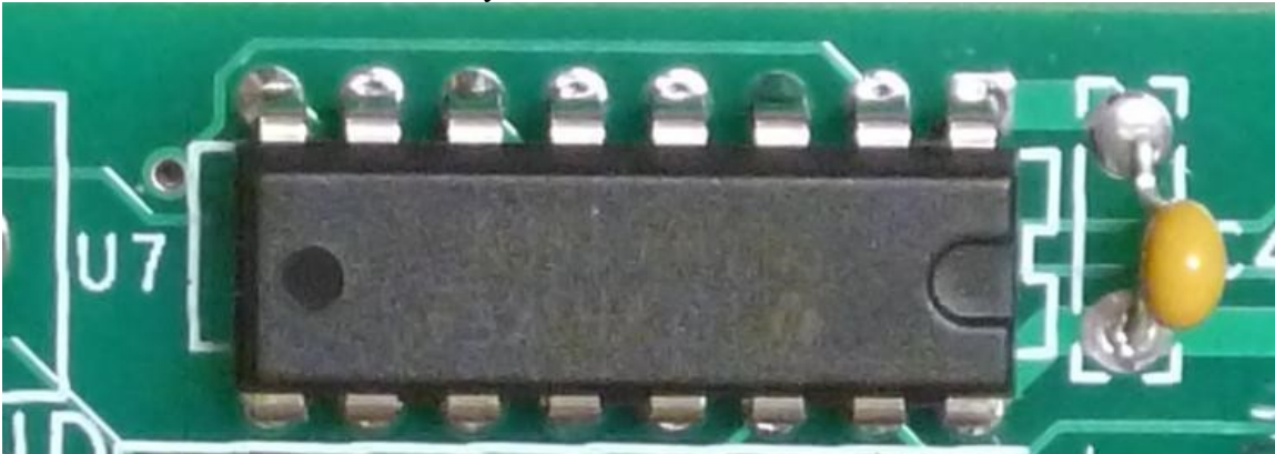
Figure 21-Insert all the IC's so that the U-shaped indent matches the silk-screen
