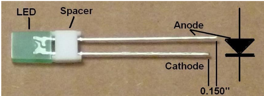
Figure 27-LED with white spacer added
