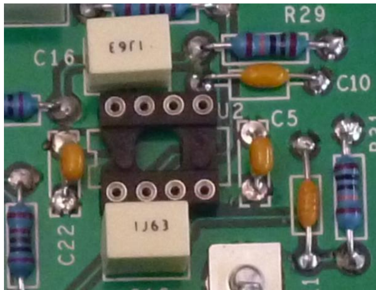
Figure 30-Align socket feature with silk screen
