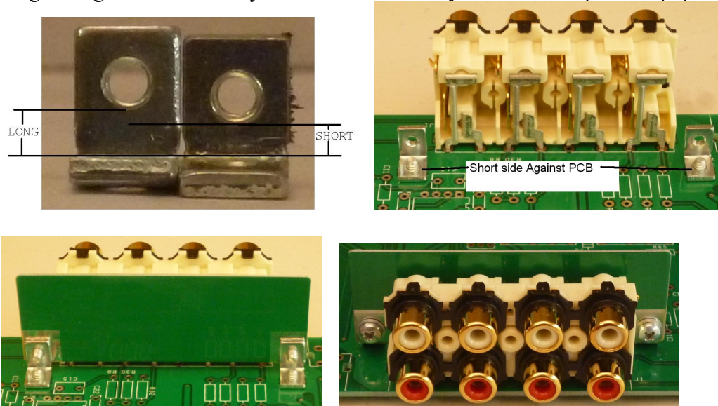
Figure 31-Mounting the input connector shield
