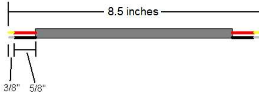
Figure 31-shielded cable for left channel. Right channel has overall length of 11 inches.
