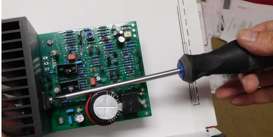
Figure 25-threading the screwdriver to Q4's mounting screw
