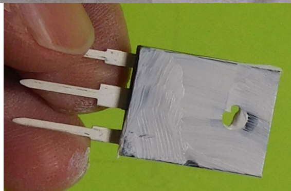
Figure 24-Spread a thin film of thermal compound on Q4 (IRFP9140), but keep it off the leads
