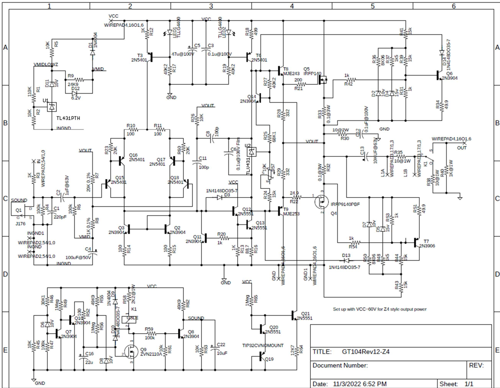
Figure 52-Amplifier Module Schematic
