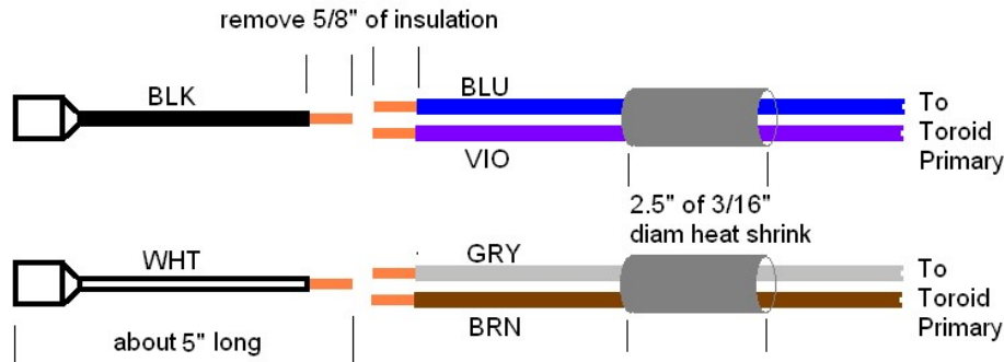
Figure 43-Wiring toroidal transformer for 120 Volt operation
